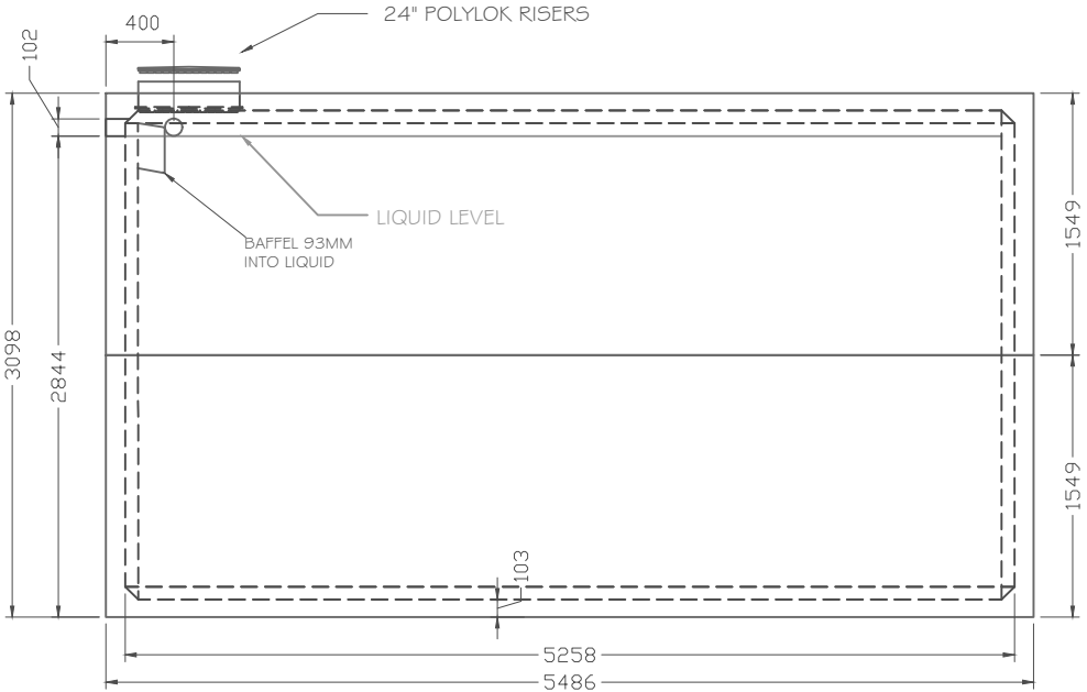
SIDE VIEW
