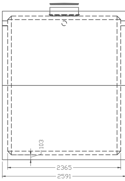
END VIEW
