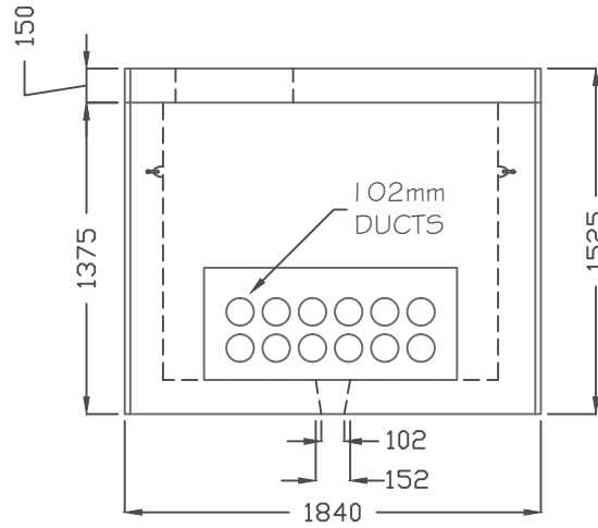
SIDE VIEW (1)
