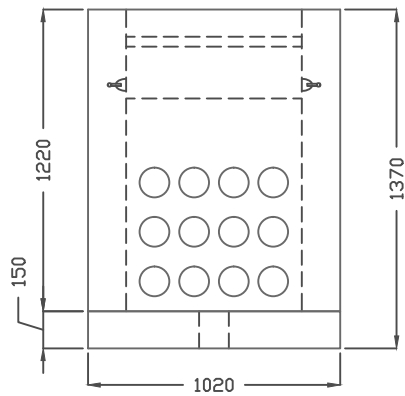
SIDE VIEW (2)
