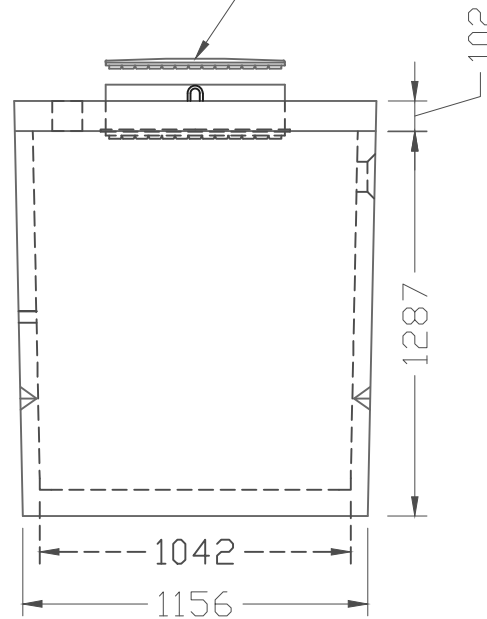
SIDE VIEW (2)
