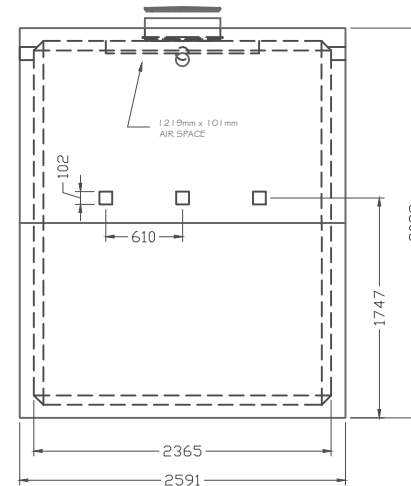
END VIEW
